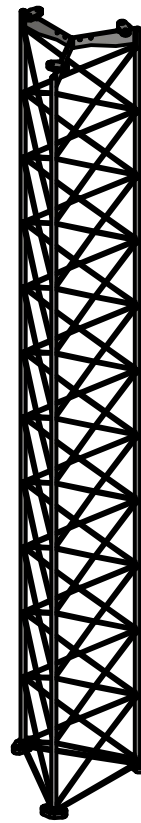
3D VIEW ( 1 : 50 )
